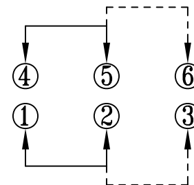
SCHEMATIC(NON-SHORTING)
